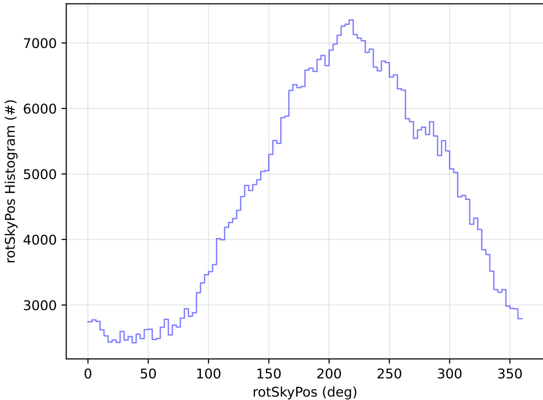
ddf_acor_sf15_lsf40_lsr20_v3.4_10yrs All sky i band: rotSkyPos Histogram
