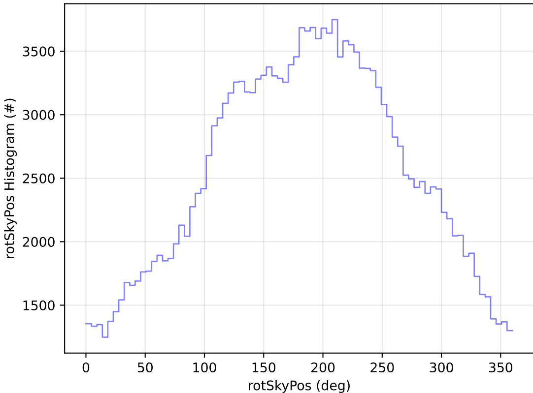
ddf_acor_sf15_lsf40_lsr20_v3.4_10yrs All sky g band: rotSkyPos Histogram
