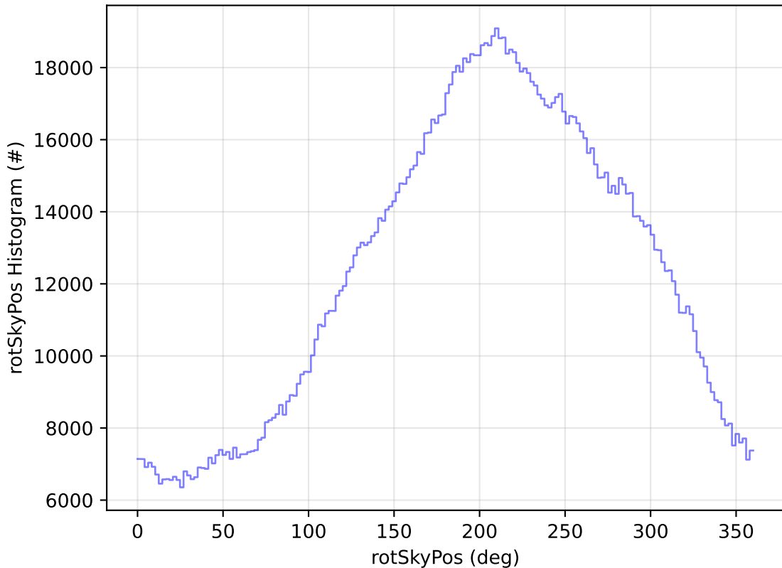
ddf_acor_sf15_lsf40_lsr20_v3.4_10yrs All sky all bands: rotSkyPos Histogram
