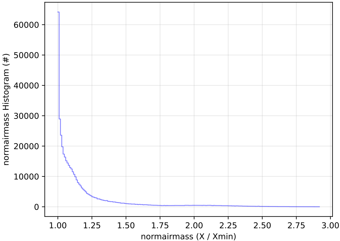
ddf_acor_sf15_lsf40_lsr20_v3.4_10yrs WFD z band: normairmass Histogram
