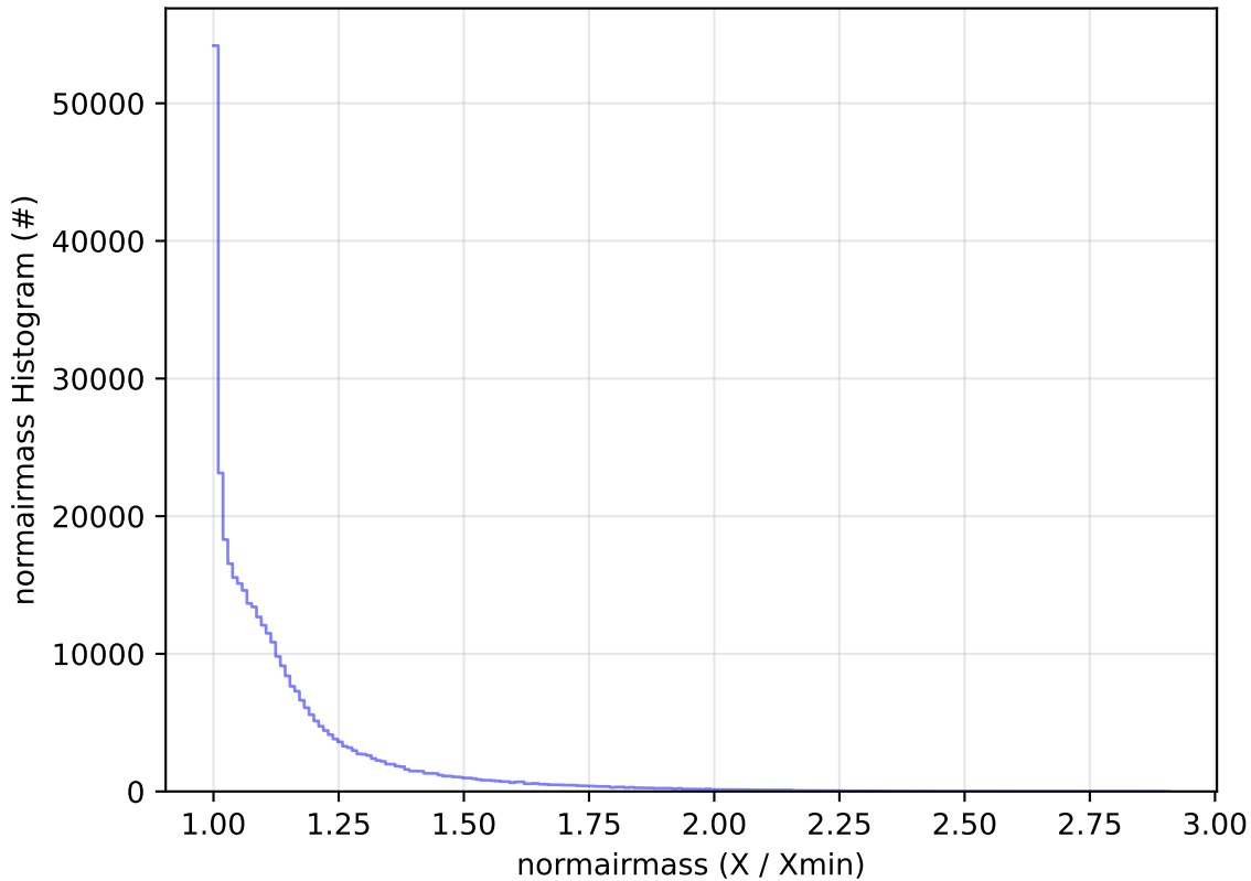
ddf_acor_sf15_lsf40_lsr20_v3.4_10yrs WFD y band: normairmass Histogram
