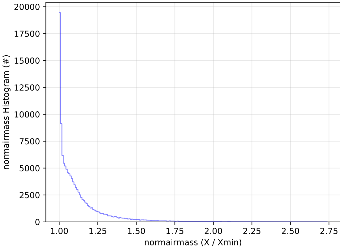
ddf_acor_sf15_lsf40_lsr20_v3.4_10yrs WFD u band: normairmass Histogram
