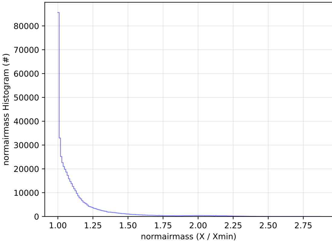
ddf_acor_sf15_lsf40_lsr20_v3.4_10yrs WFD r band: normairmass Histogram
