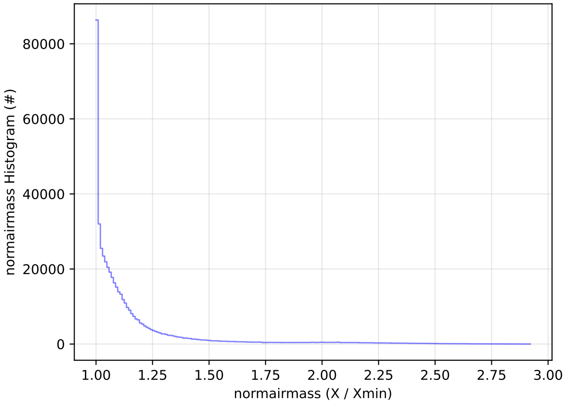
ddf_acor_sf15_lsf40_lsr20_v3.4_10yrs WFD i band: normairmass Histogram
