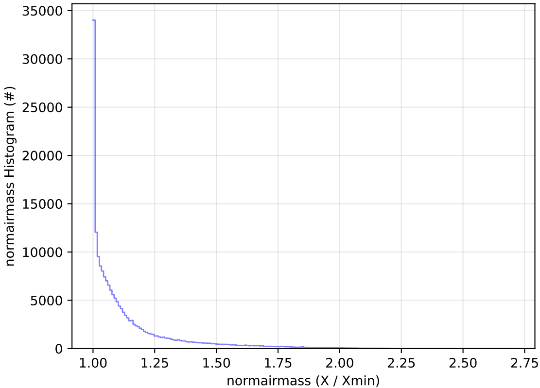
ddf_acor_sf15_lsf40_lsr20_v3.4_10yrs WFD g band: normairmass Histogram
