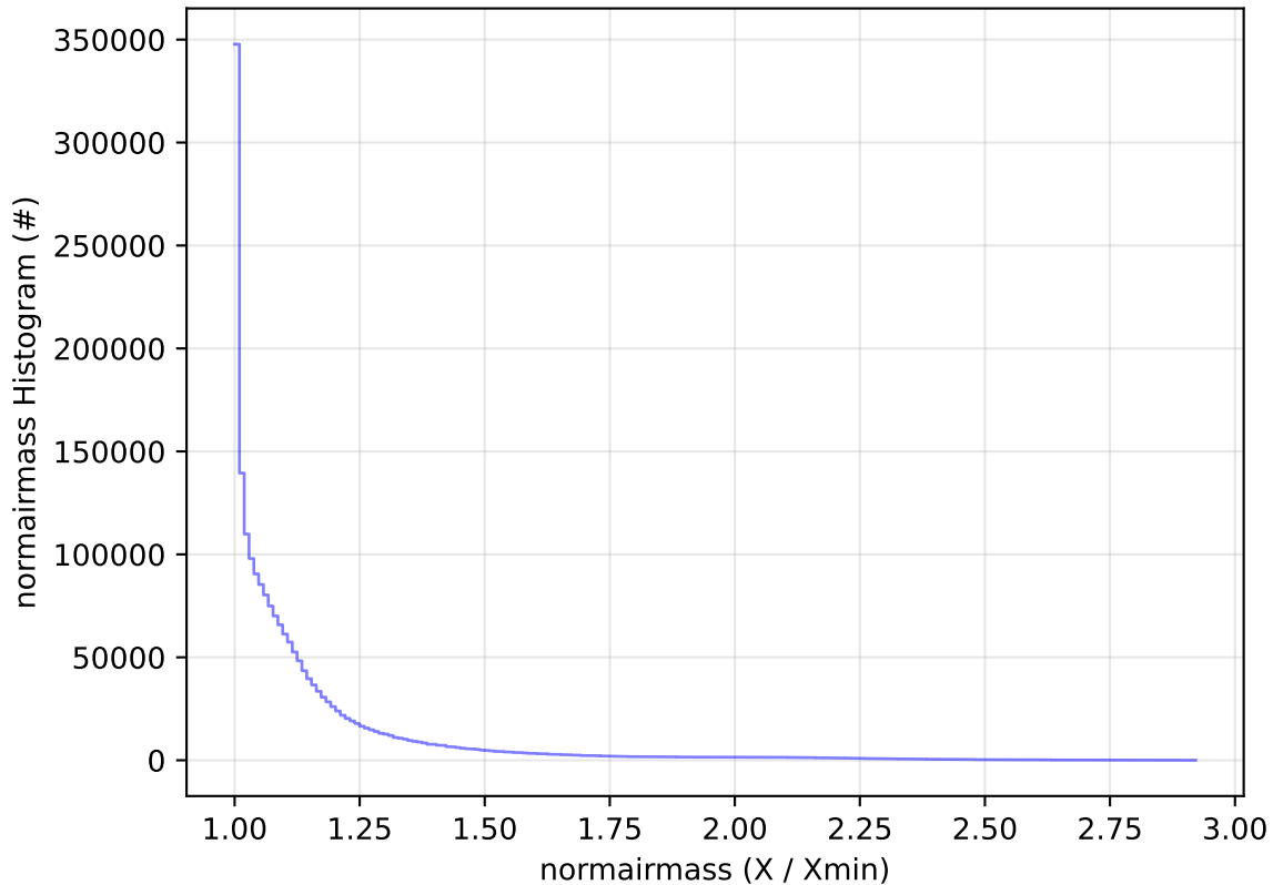
ddf_acor_sf15_lsf40_lsr20_v3.4_10yrs WFD all bands: normairmass Histogram
