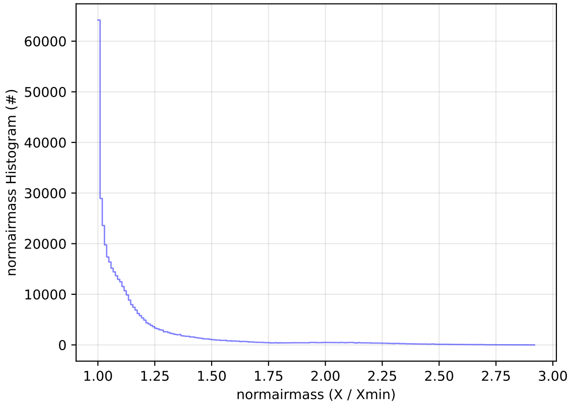
ddf_acor_sf15_lsf40_lsr20_v3.4_10yrs All sky z band: normairmass Histogram
