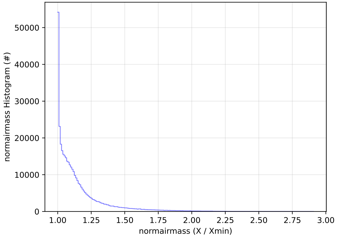
ddf_acor_sf15_lsf40_lsr20_v3.4_10yrs All sky y band: normairmass Histogram
