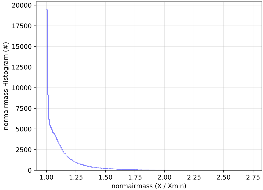
ddf_acor_sf15_lsf40_lsr20_v3.4_10yrs All sky u band: normairmass Histogram
