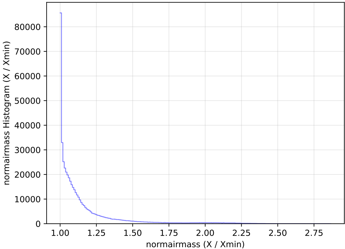
ddf_acor_sf15_lsf40_lsr20_v3.4_10yrs All sky r band: normairmass Histogram
