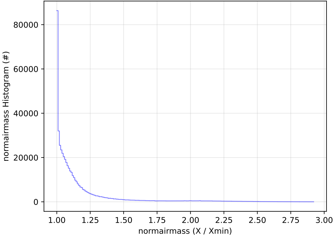
ddf_acor_sf15_lsf40_lsr20_v3.4_10yrs All sky i band: normairmass Histogram
