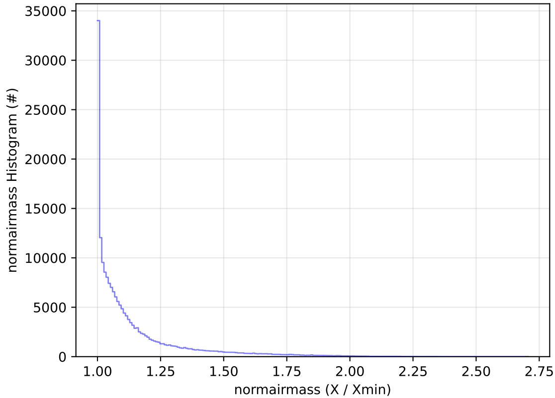
ddf_acor_sf15_lsf40_lsr20_v3.4_10yrs All sky g band: normairmass Histogram
