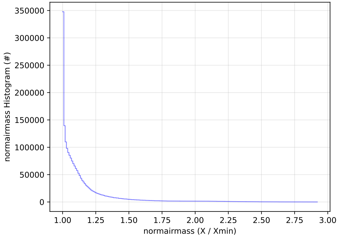
ddf_acor_sf15_lsf40_lsr20_v3.4_10yrs All sky all bands: normairmass Histogram
