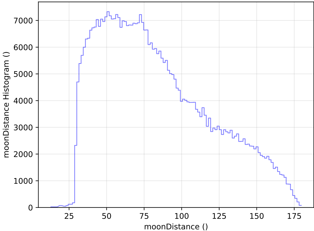
ddf_acor_sf15_ls40_lsr20_v3.4_10yrs WFD z band: moonDistance Histogram
