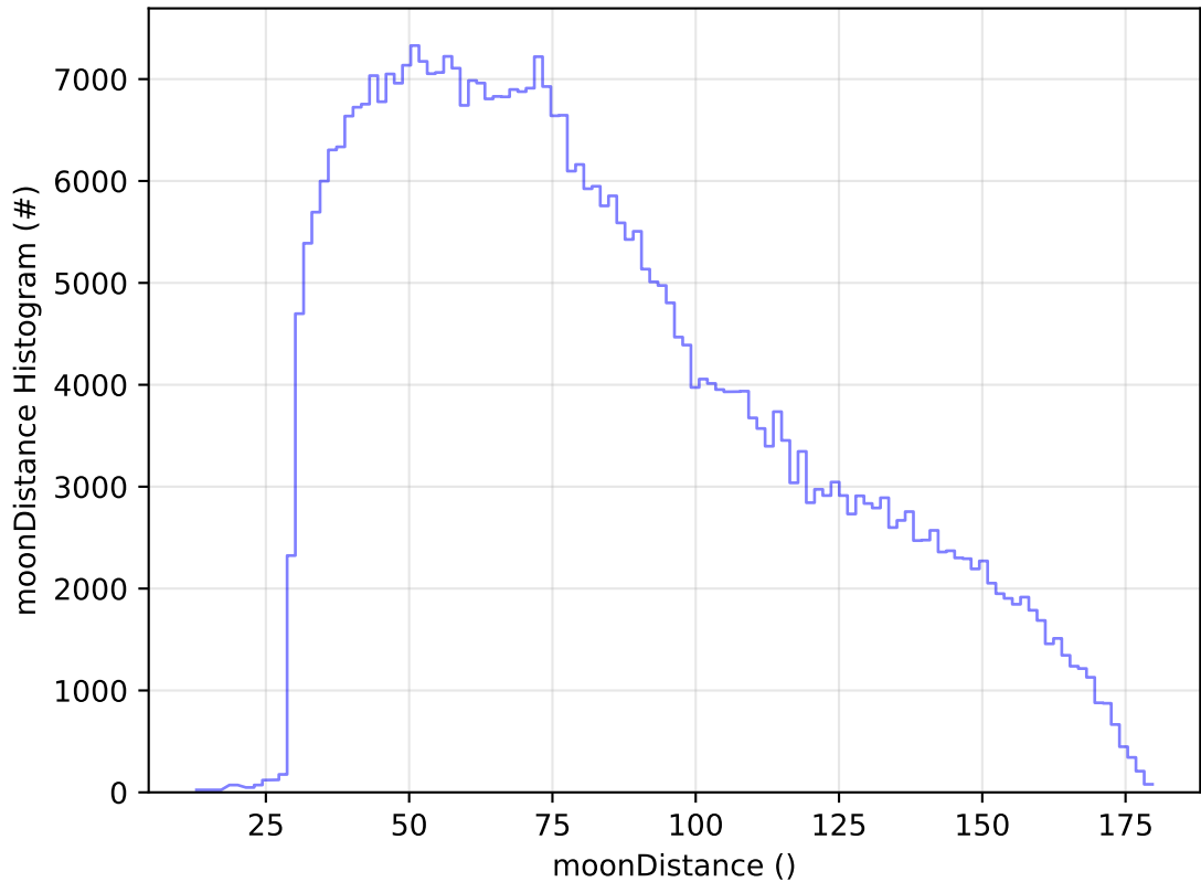
ddf_acor_sf15_lsf40_lsr20_v3.4_10yrs WFD z band: moonDistance Histogram
