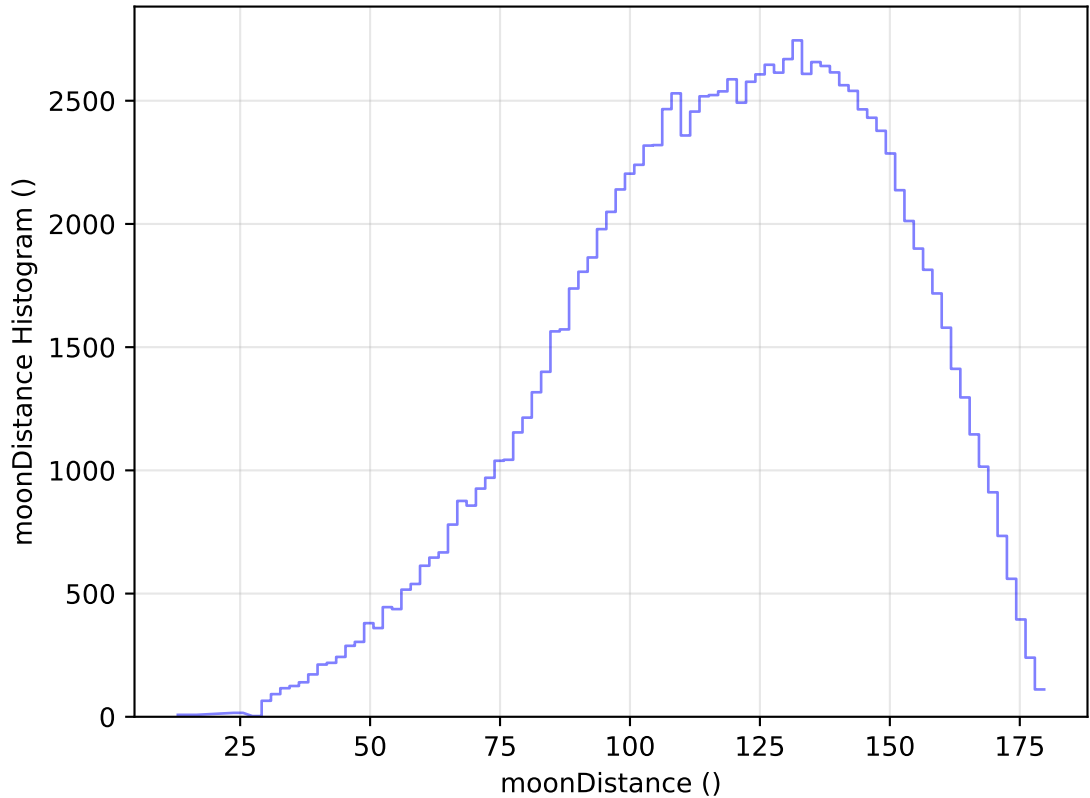
ddf_acor_sf15_lsf40_lsr20_v3.4_10yrs WFD u band: moonDistance Histogram
