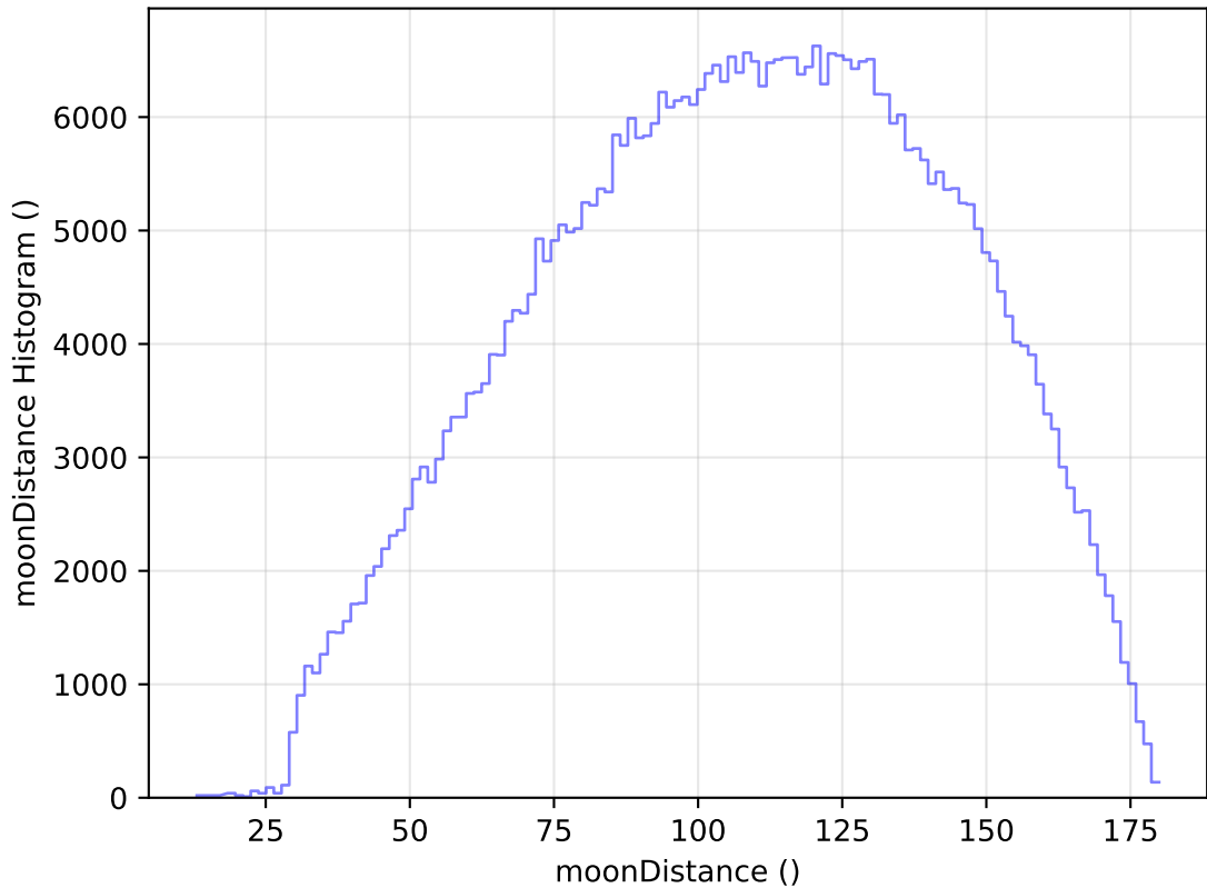
ddf_acor_sf15_lsf40_lsr20_v3.4_10yrs WFD r band: moonDistance Histogram
