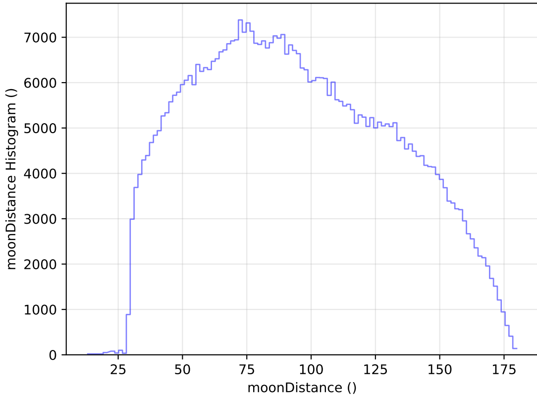
ddf_acor_sf15_lsf40_lsr20_v3.4_10yrs WFD i band: moonDistance Histogram
