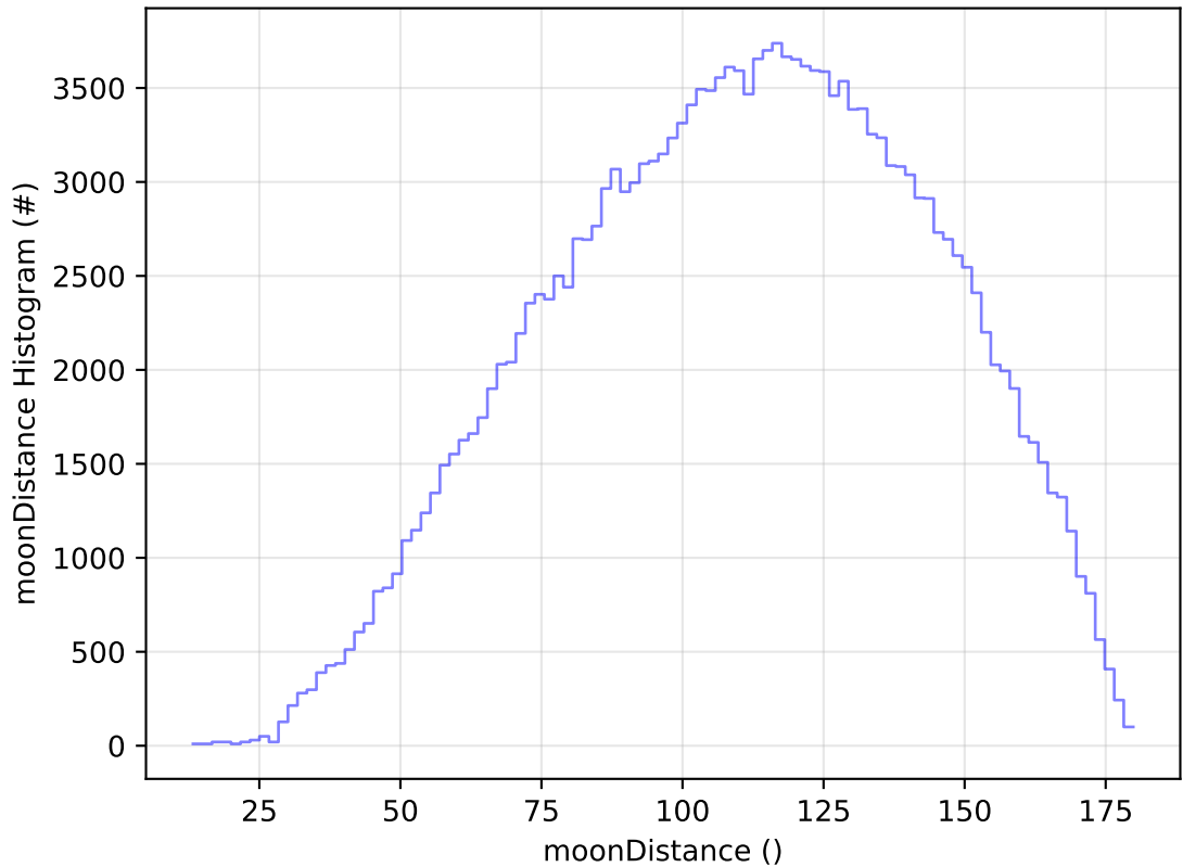
ddf_acor_sf15_lsf40_lsr20_v3.4_10yrs WFD g band: moonDistance Histogram
