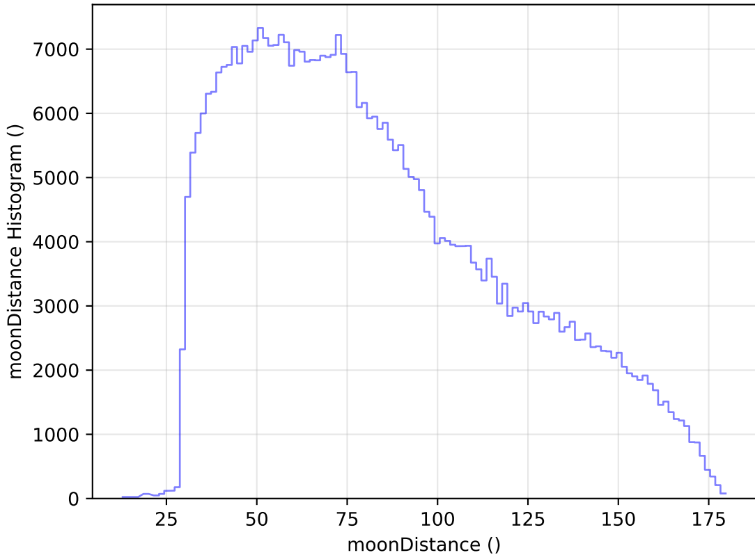
ddf_acor_sf15_lsf40_lsr20_v3.4_10yrs All sky z band: moonDistance Histogram
