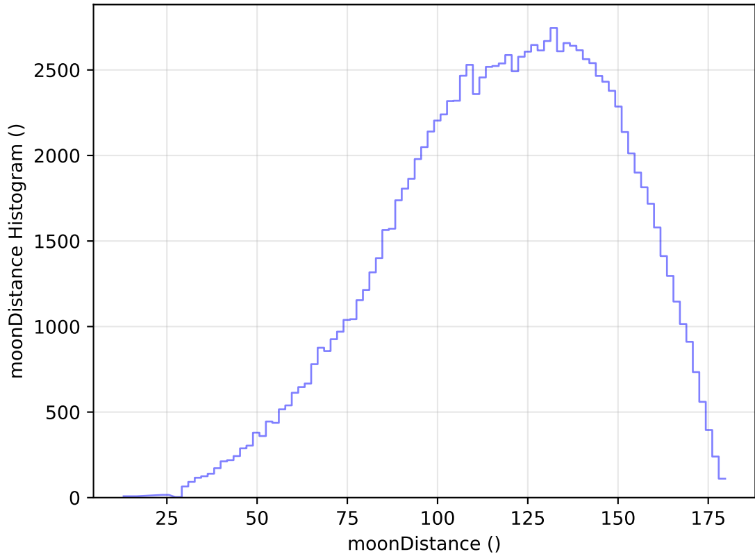
ddf_acor_sf15_lsf40_lsr20_v3.4_10yrs All sky u band: moonDistance Histogram
