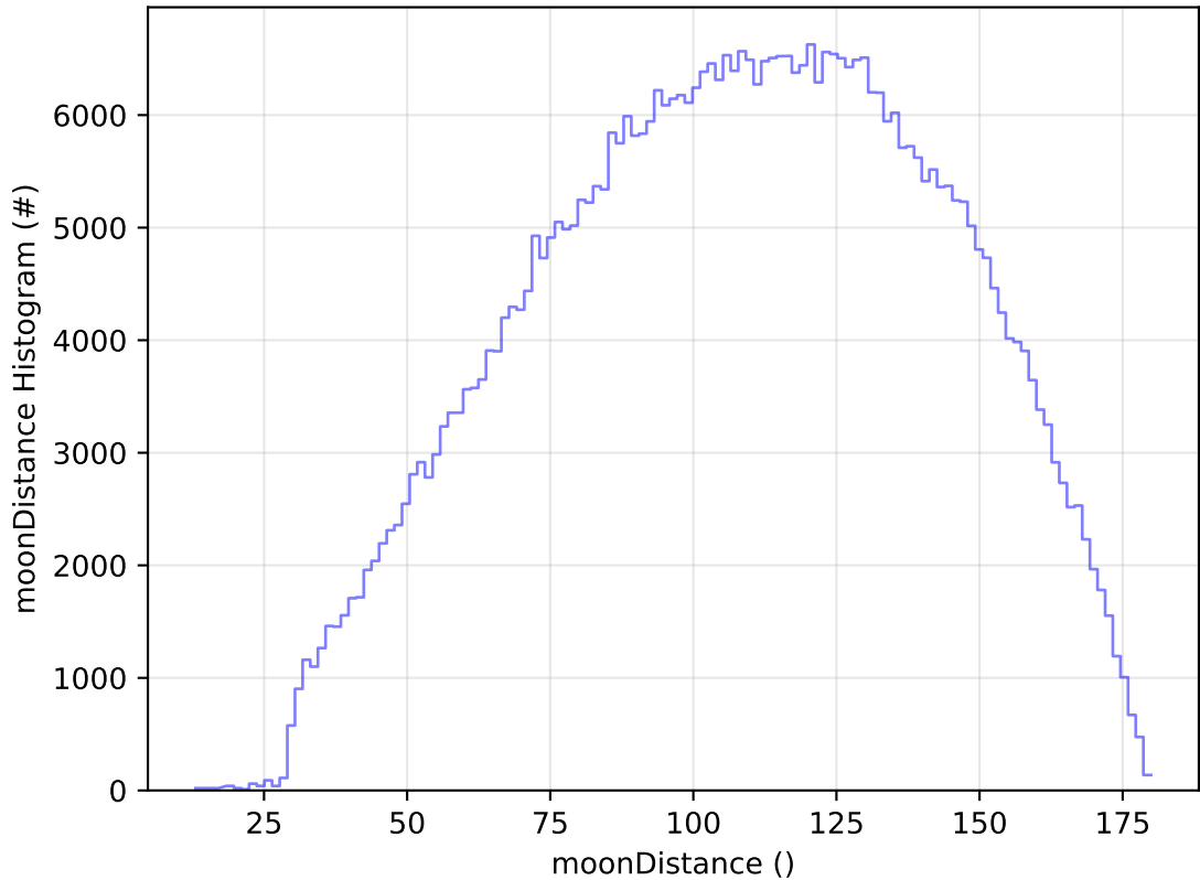
ddf_acor_sf15_lsf40_lsr20_v3.4_10yrs All sky r band: moonDistance Histogram
