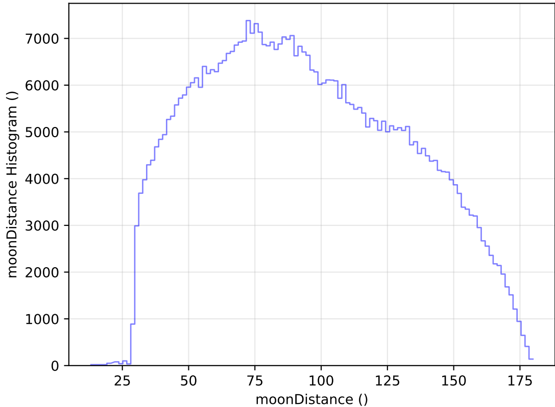
ddf_acor_sf15_lsf40_lsr20_v3.4_10yrs All sky i band: moonDistance Histogram
