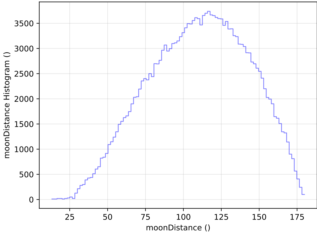
ddf_acor_sf15_lsf40_lsr20_v3.4_10yrs All sky g band: moonDistance Histogram
