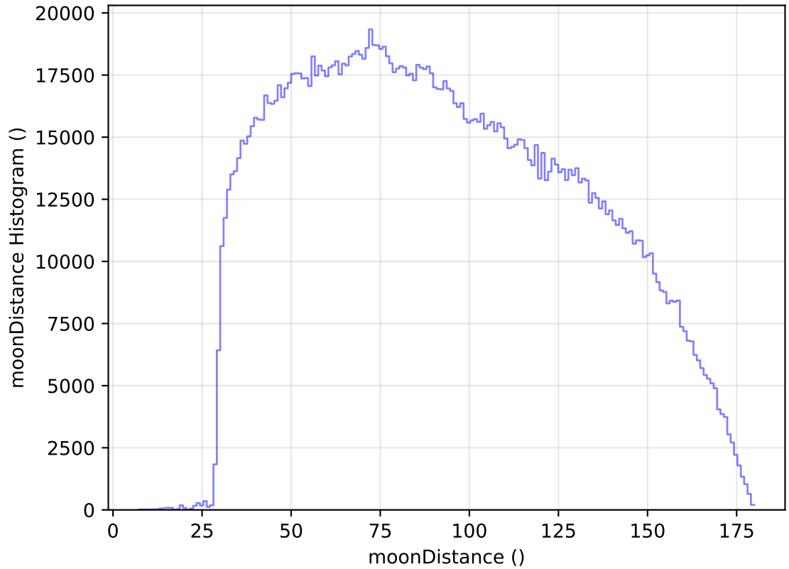
ddf_acor_sf15_lsf40_lsr20_v3.4_10yrs All sky all bands: moonDistance Histogram
