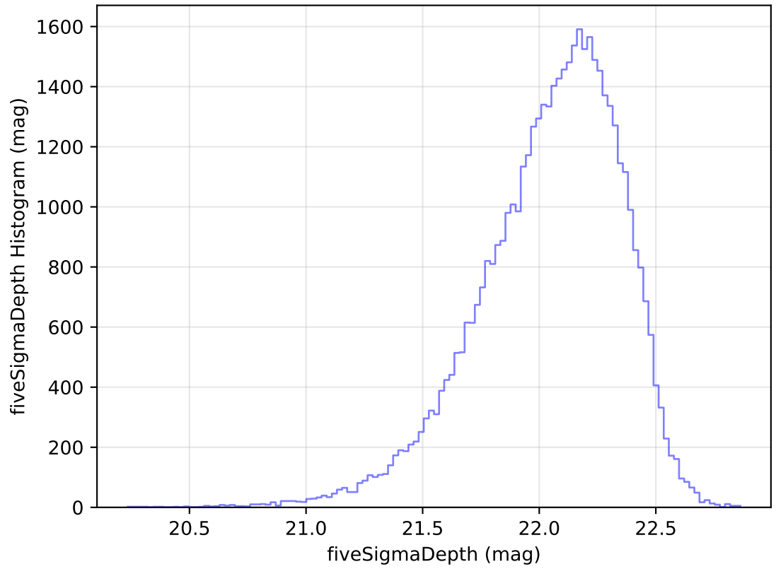
ddf_acor_sf15_lsf40_lsr20_v3.4_10yrs Yr 1 y band: fiveSigmaDepth Histogram
