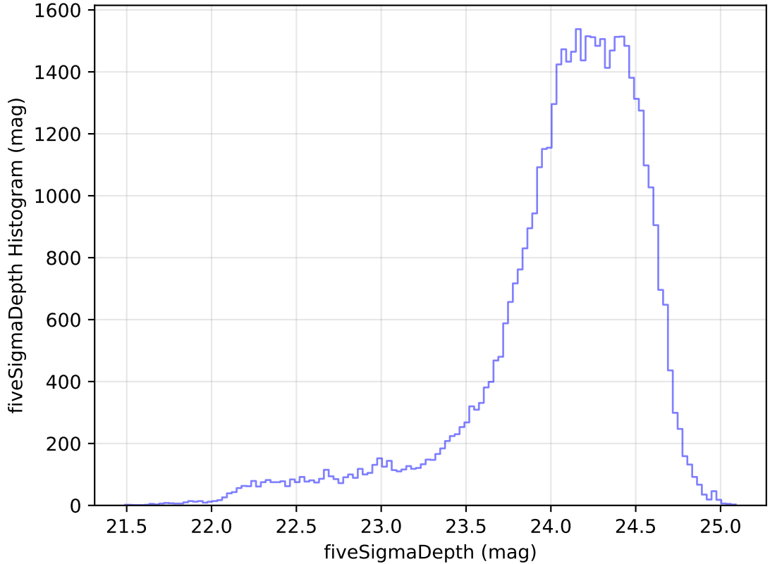
ddf_acor_sf15_lsf40_lsr20_v3.4_10yrs Yr 1 r band: fiveSigmaDepth Histogram
