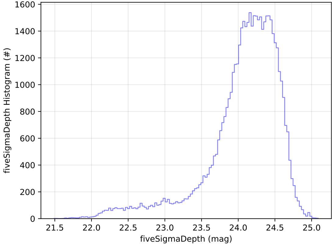
ddf_acor_sf15_ls40_lsr20_v3.4_10yrs Yr 1 r band: fiveSigmaDepth Histogram
