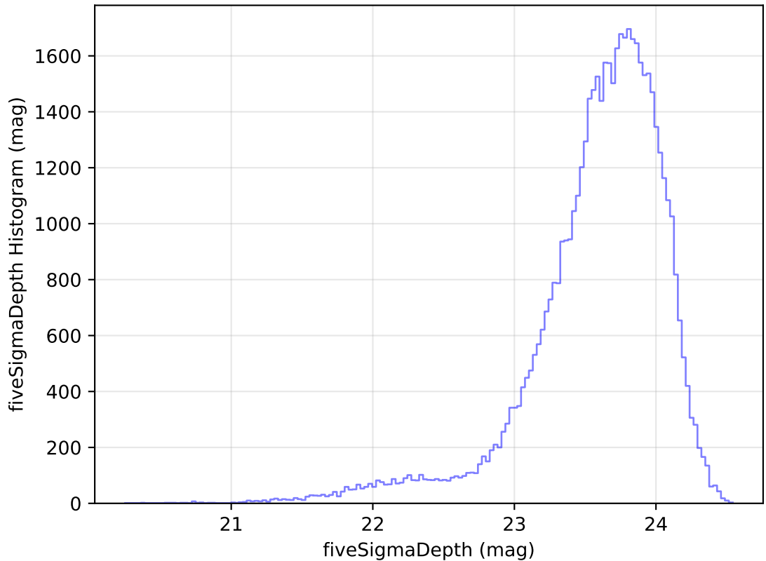
ddf_acor_sf15_lsf40_lsr20_v3.4_10yrs Yr 1 i band: fiveSigmaDepth Histogram
