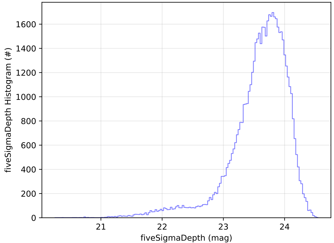
ddf_acor_sf15_lsf40_lsr20_v3.4_10yrs Yr 1 i band: fiveSigmaDepth Histogram
