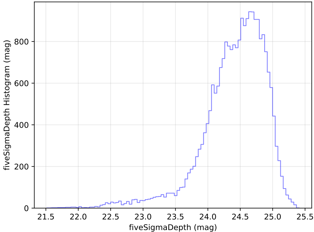
ddf_acor_sf15_lsf40_lsr20_v3.4_10yrs Yr 1 g band: fiveSigmaDepth Histogram
