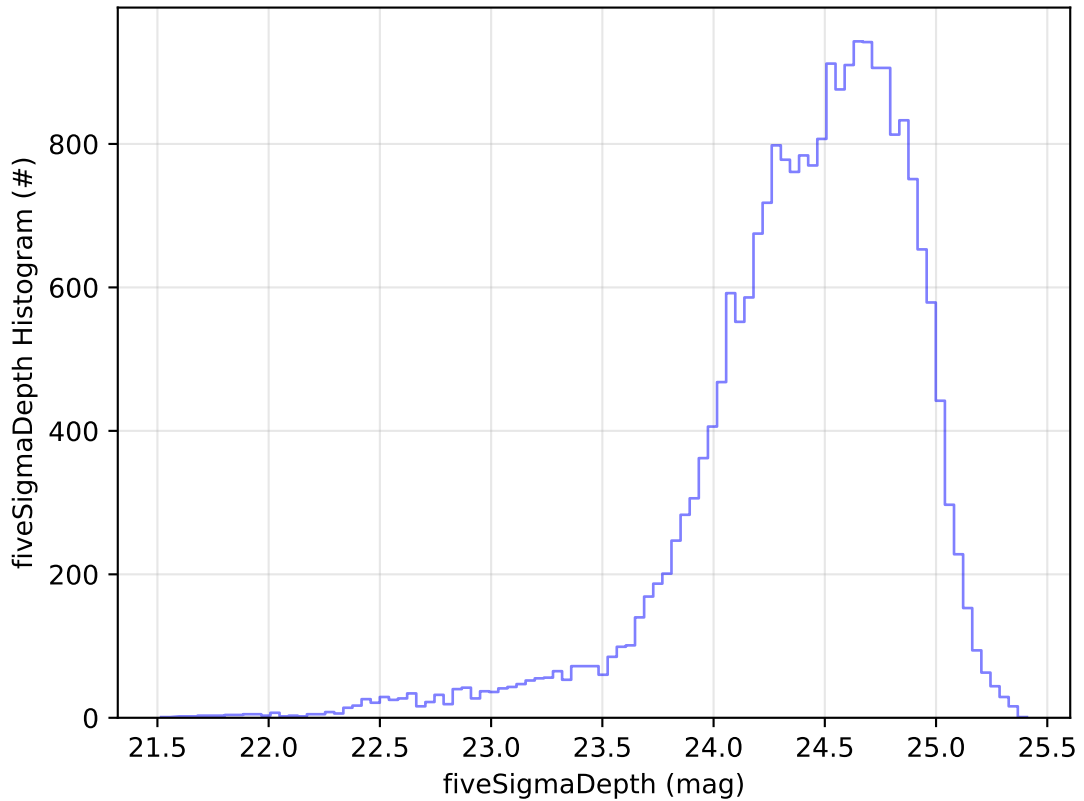
ddf_acor_sf15_lsf40_lsr20_v3.4_10yrs Yr 1 g band: fiveSigmaDepth Histogram
