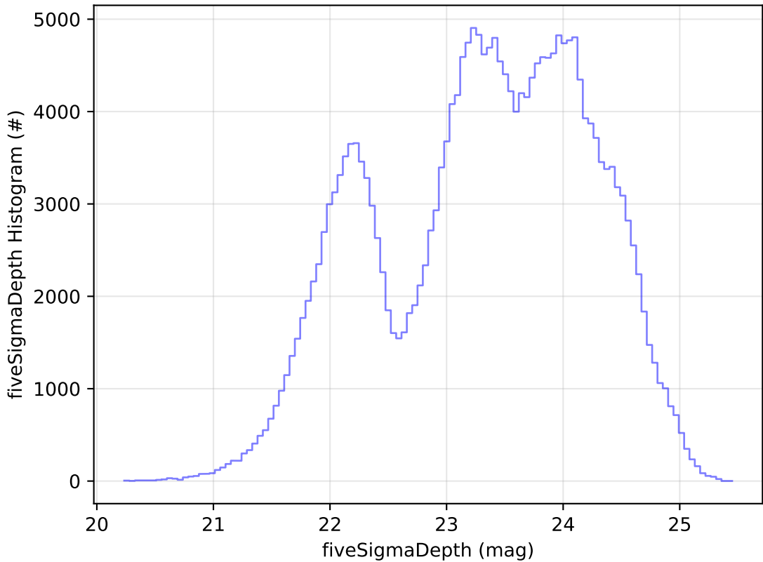
ddf_acor_sf15_lsf40_lsr20_v3.4_10yrs Yr 1 all bands: fiveSigmaDepth Histogram
