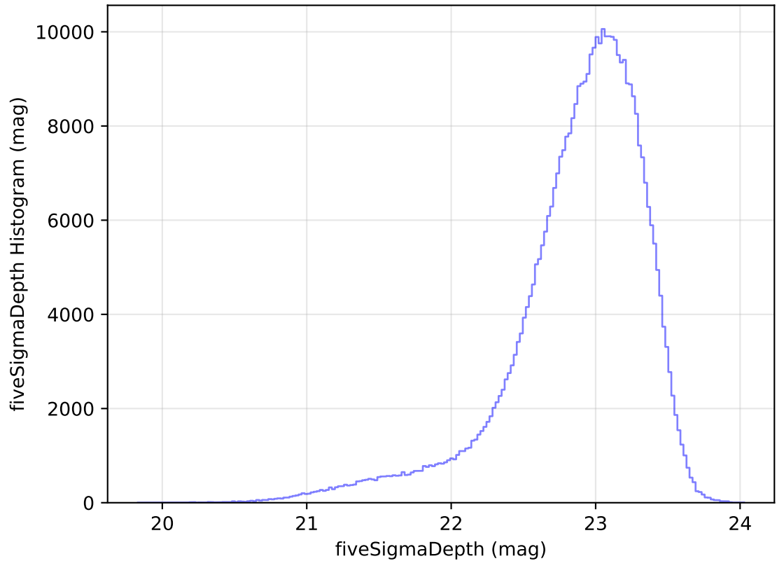
ddf_acor_sf15_lsf40_lsr20_v3.4_10yrs WFD z band: fiveSigmaDepth Histogram
