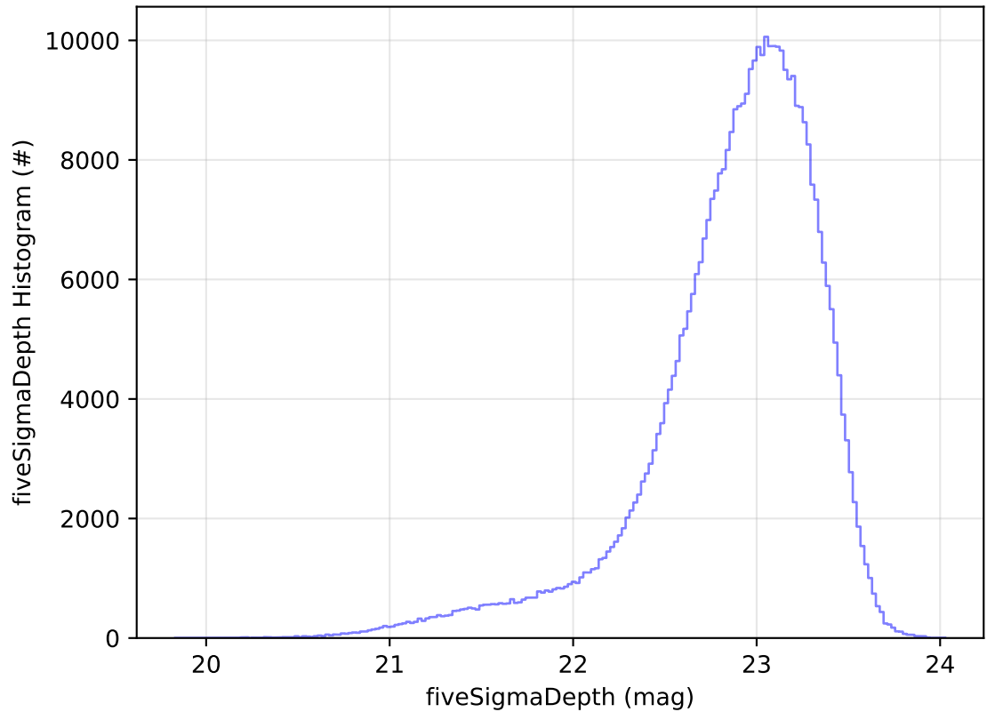
ddf_acor_sf15_ls40_lsr20_v3.4_10yrs WFD z band: fiveSigmaDepth Histogram
