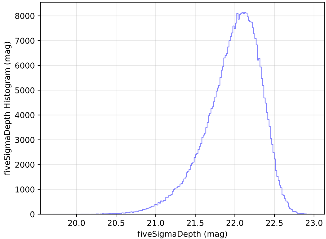
ddf_acor_sf15_lsf40_lsr20_v3.4_10yrs WFD y band: fiveSigmaDepth Histogram
