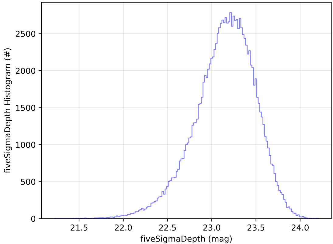
ddf_acor_sf15_lsf40_lsr20_v3.4_10yrs WFD u band: fiveSigmaDepth Histogram
