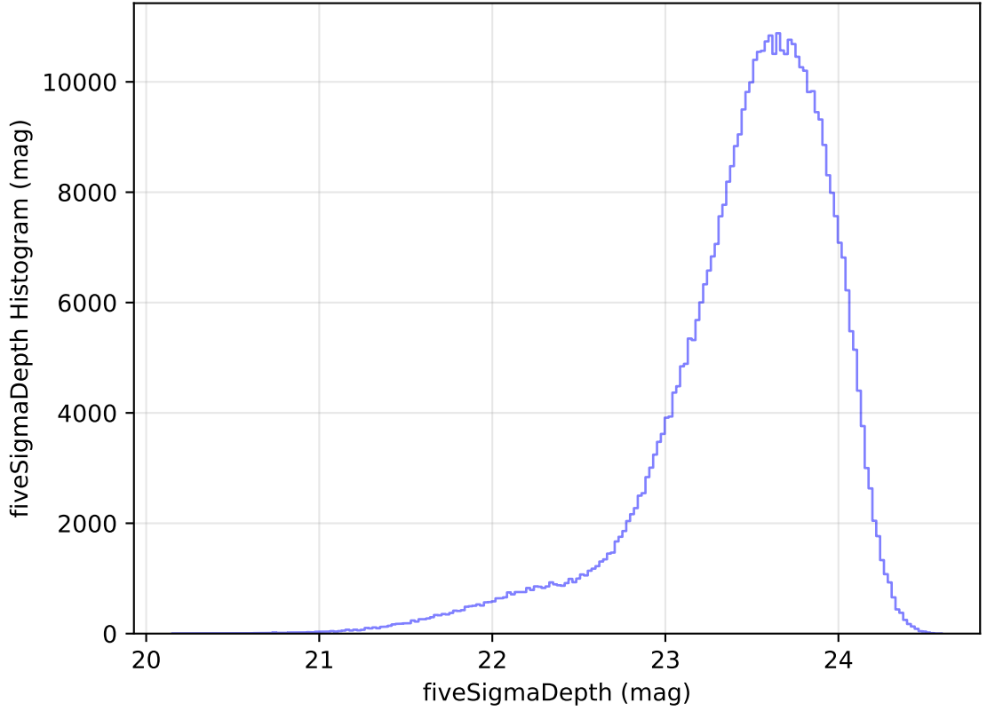
ddf_acor_sf15_lsf40_lsr20_v3.4_10yrs WFD i band: fiveSigmaDepth Histogram
