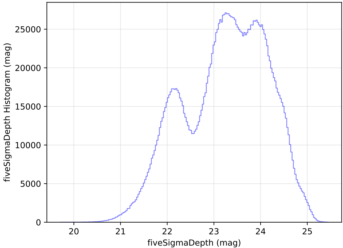
ddf_acor_sf15_lsf40_lsr20_v3.4_10yrs WFD all bands: fiveSigmaDepth Histogram
