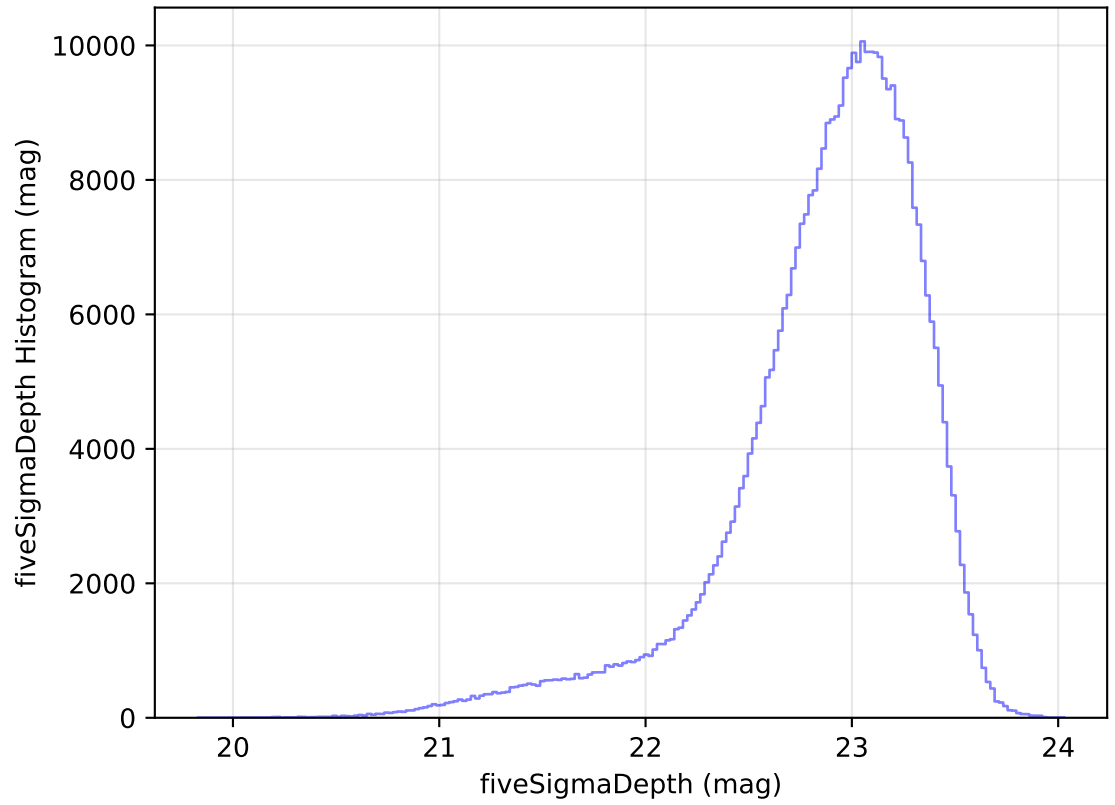
ddf_acor_sf15_ls40_lsr20_v3.4_10yrs All sky z band: fiveSigmaDepth Histogram
