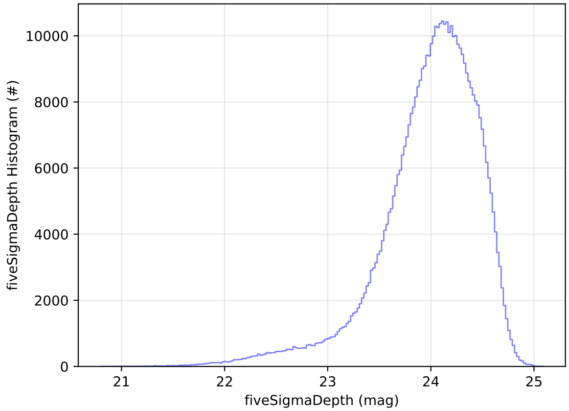
ddf_acor_sf15_lsf40_lsr20_v3.4_10yrs All sky r band: fiveSigmaDepth Histogram
