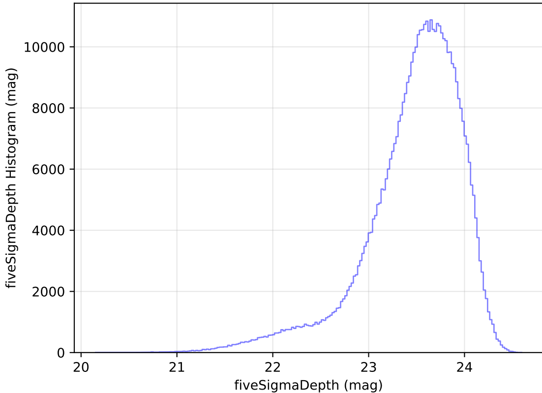
ddf_acor_sf15_lsf40_lsr20_v3.4_10yrs All sky i band: fiveSigmaDepth Histogram
