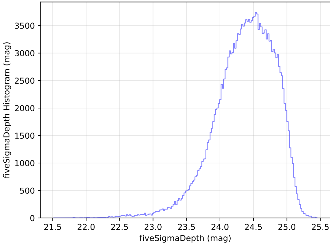
ddf_acor_sf15_lsf40_lsr20_v3.4_10yrs All sky g band: fiveSigmaDepth Histogram
