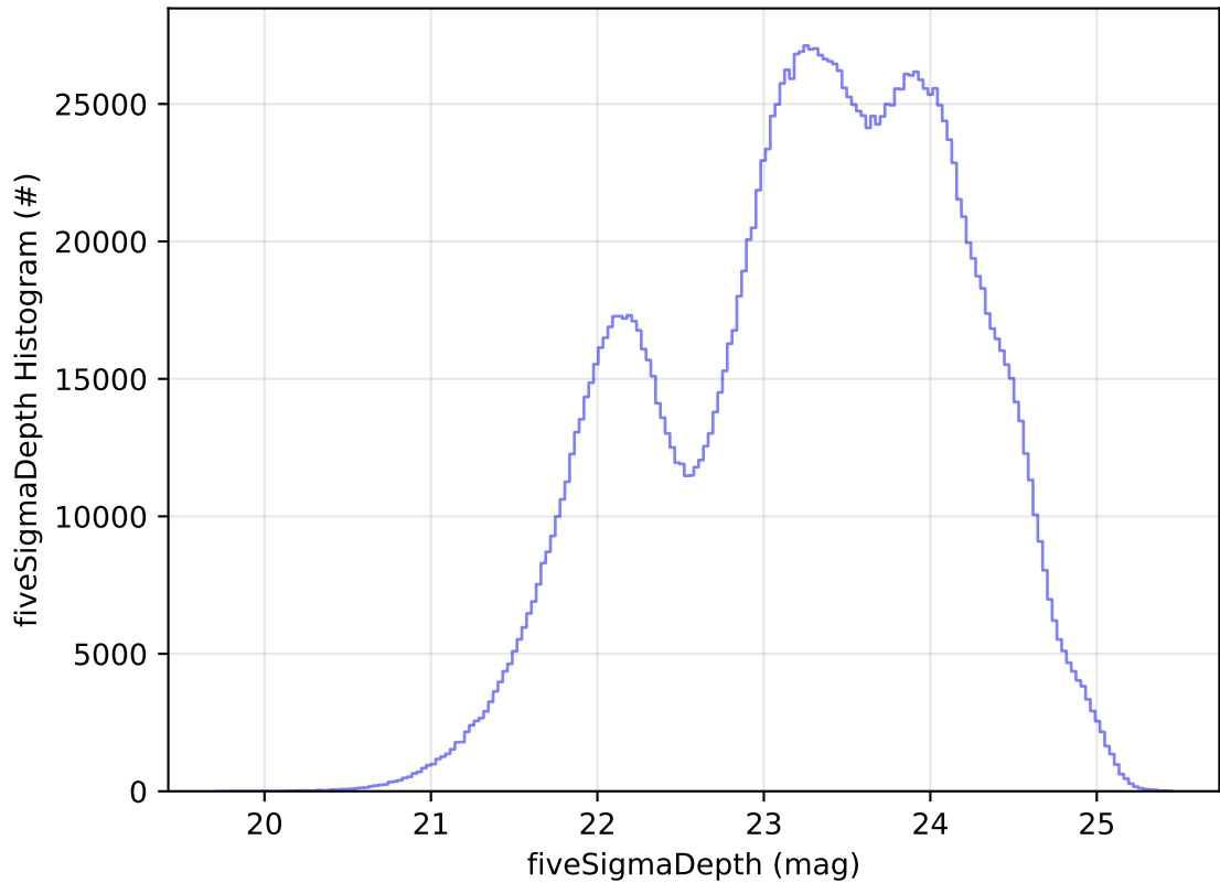
ddf_acor_sf15_lsf40_lsr20_v3.4_10yrs All sky all bands: fiveSigmaDepth Histogram
