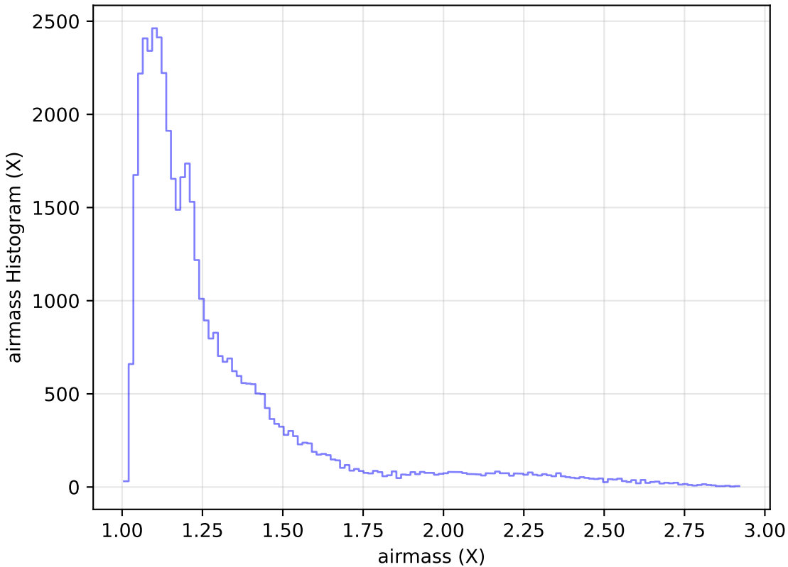
ddf_acor_sf15_ls40_lsr20_v3.4_10yrs Yr 1 z band: airmass Histogram
