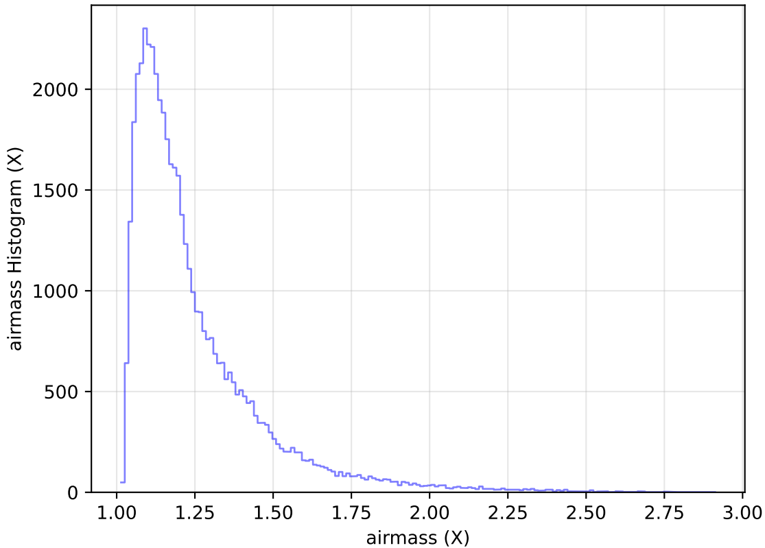
ddf_acor_sf15_ls40_lsr20_v3.4_10yrs Yr 1 y band: airmass Histogram
