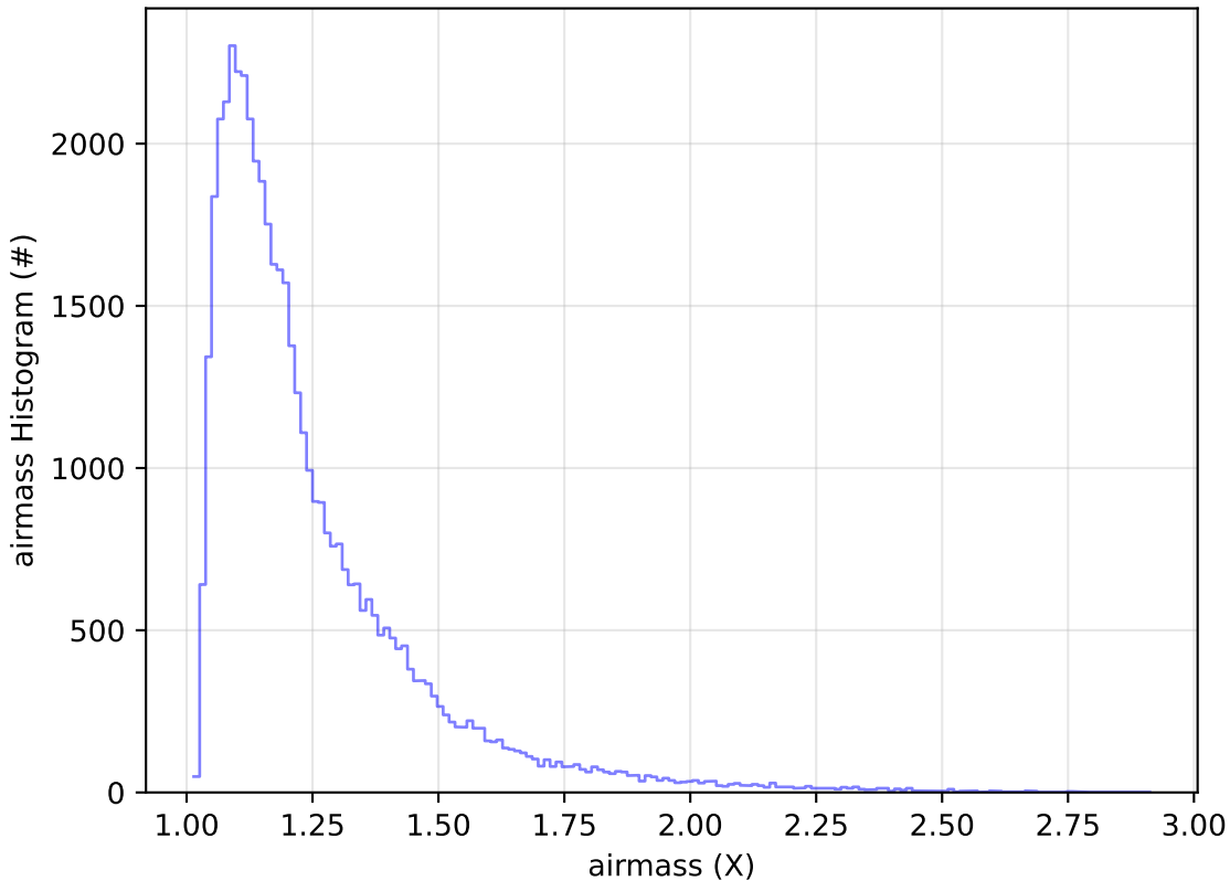
ddf_acor_sf15_lsf40_lsr20_v3.4_10yrs Yr 1 y band: airmass Histogram
