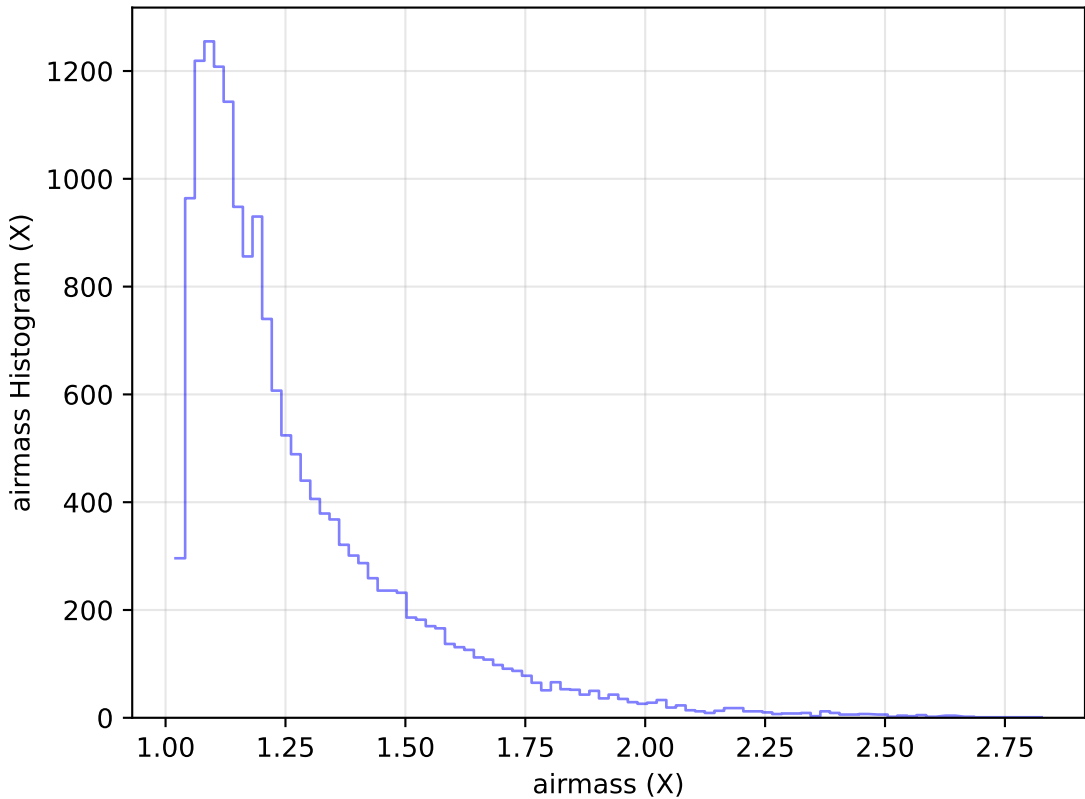
ddf_acor_sf15_lsf40_lsr20_v3.4_10yrs Yr 1 u band: airmass Histogram
