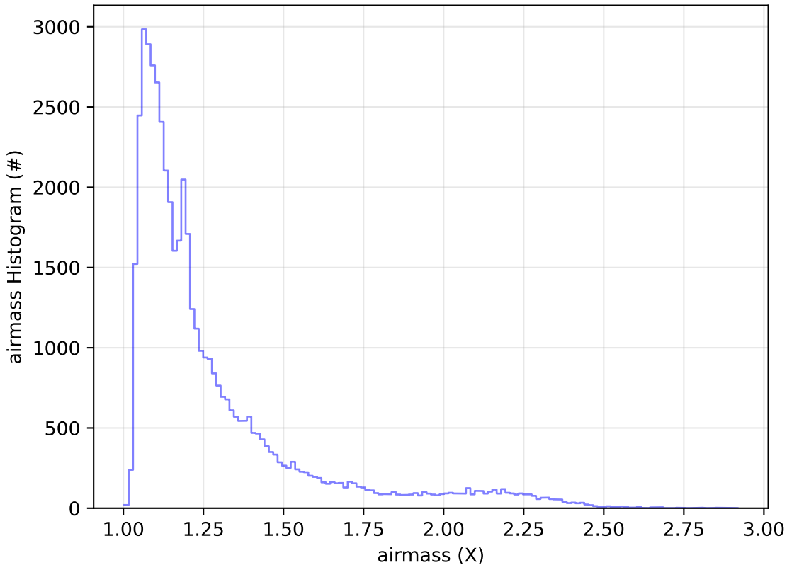
ddf_acor_sf15_Isf40_Isr20_v3.4_10yrs Yr 1 r band: airmass Histogram
