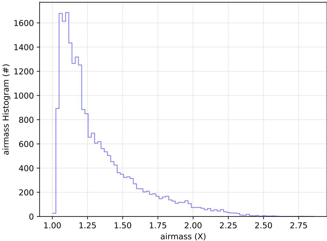
ddf_acor_sf15_lsf40_lsr20_v3.4_10yrs Yr 1 g band: airmass Histogram
