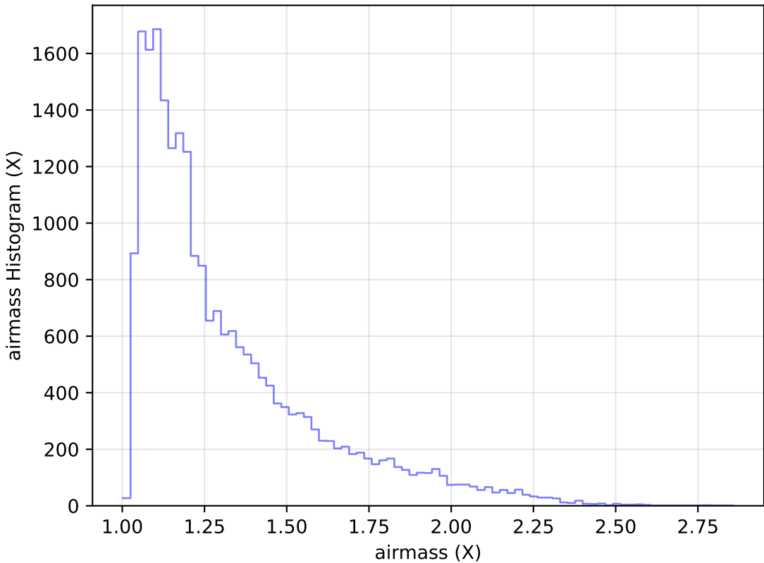
ddf_acor_sf15_ls40_lsr20_v3.4_10yrs Yr 1 g band: airmass Histogram
