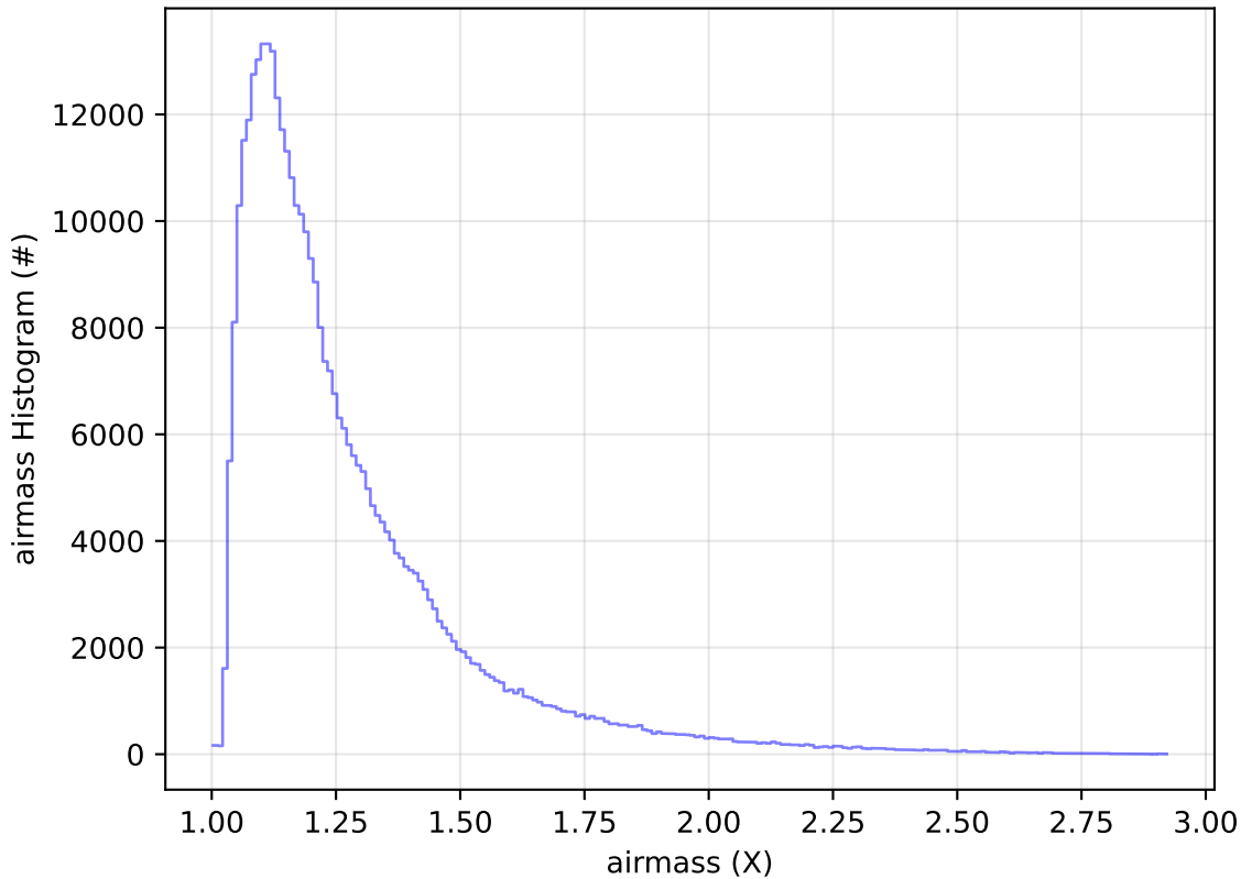
ddf_acor_sf15_lsf40_lsr20_v3.4_10yrs WFD y band: airmass Histogram
