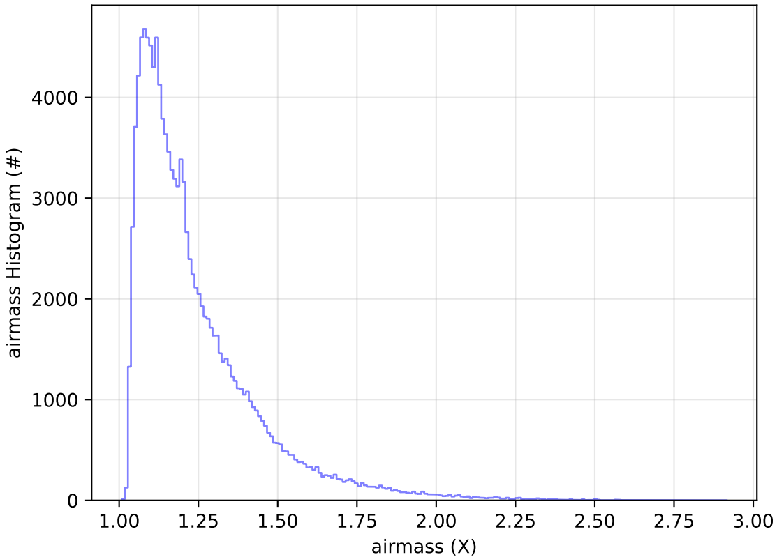
ddf_acor_sf15_lsf40_lsr20_v3.4_10yrs WFD u band: airmass Histogram
